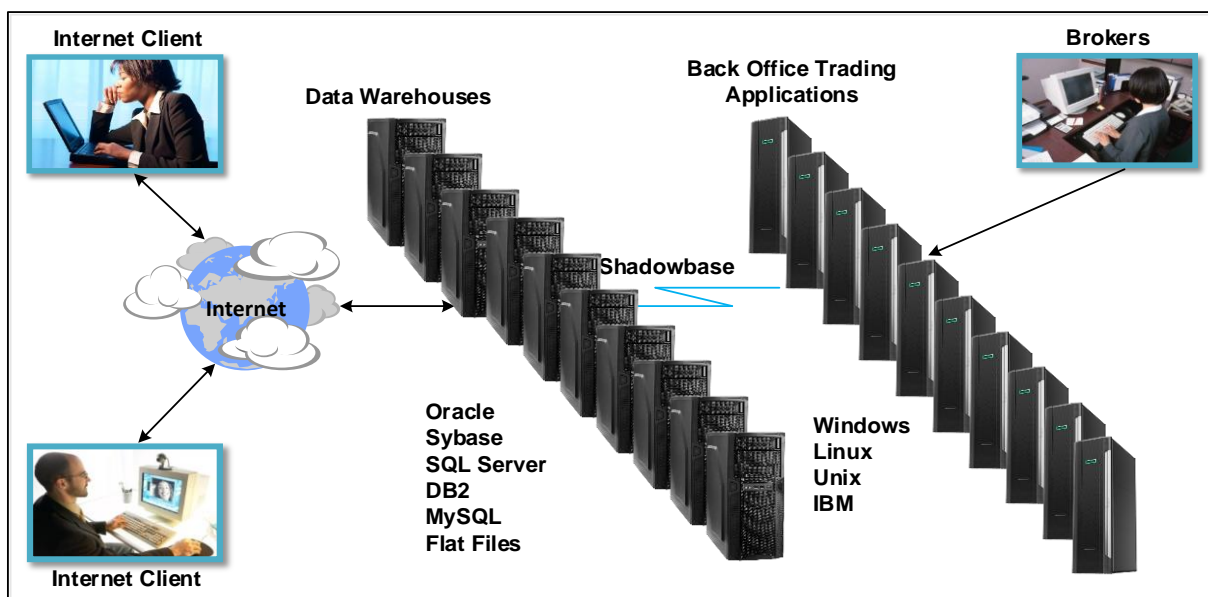
Figure 10 – HPE Shadowbase Streams Integrates HPE NonStop Trading Applications with Brokerage Data Warehouses in a Service Bureau Environment
