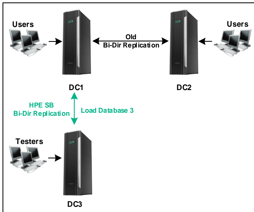
Figure 7 – Add the DC3 Node
