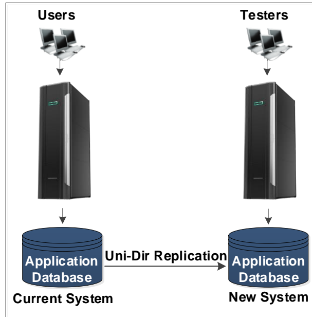
Figure 3 – HPE Shadowbase ZDM Step 3
