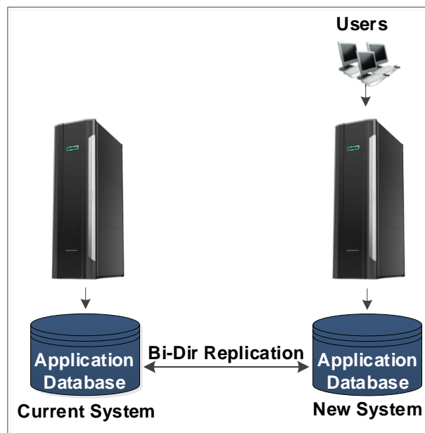
Figure 4 – HPE Shadowbase ZDM Step 4
