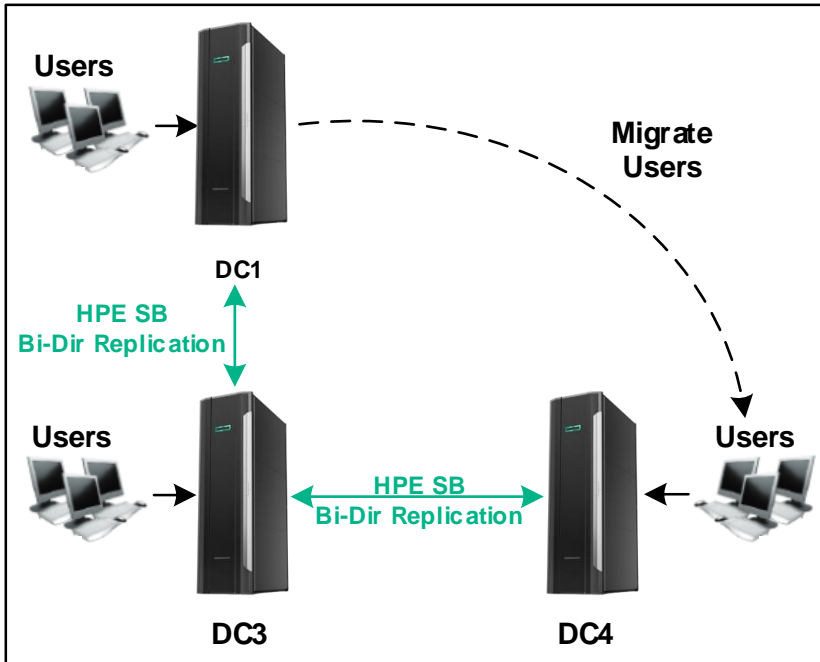
Figure 12 – Migrate Users from DC1 to DC4
