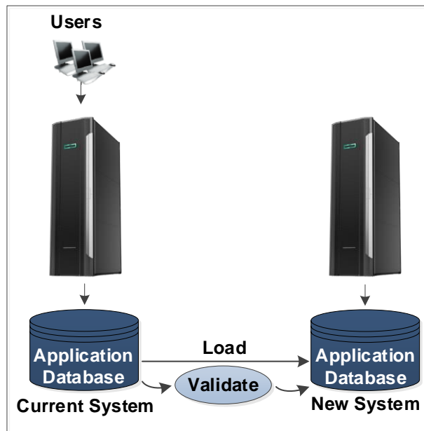
Figure 2 – HPE Shadowbase ZDM Step 2
