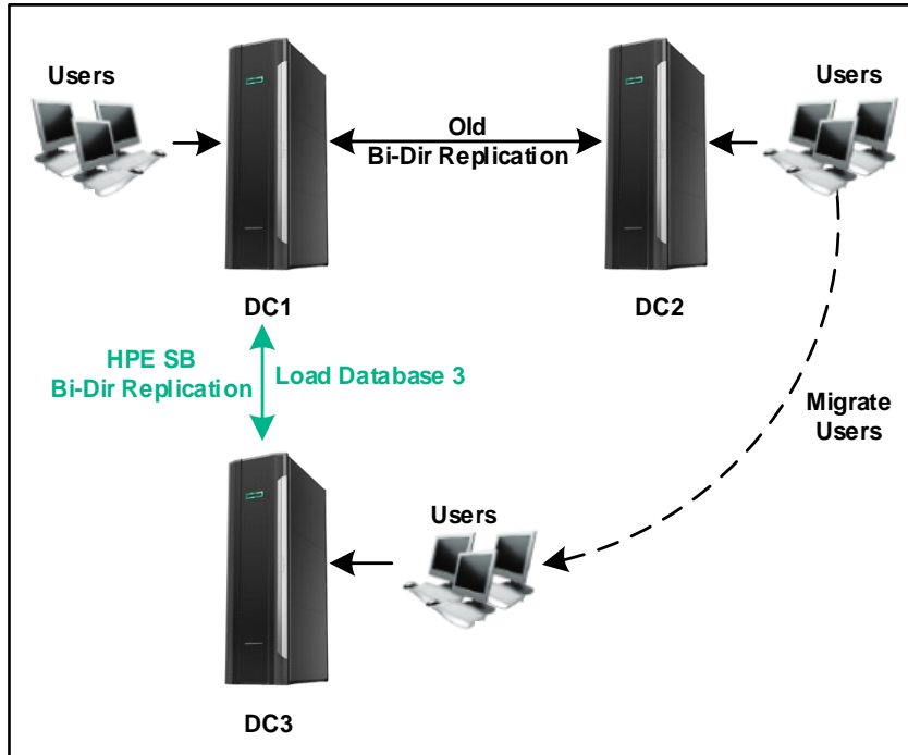
Figure 8 – Migrate Users from DC2 to DC3
