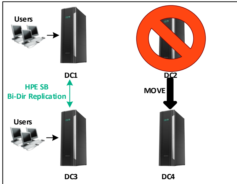
Figure 10 – Shutdown, Move, and Rename DC2 to DC4
